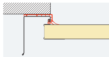
Side sealing
