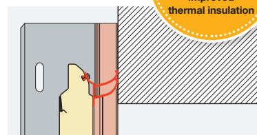
Lintel sealing
