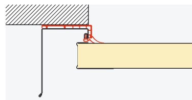
Side sealing
