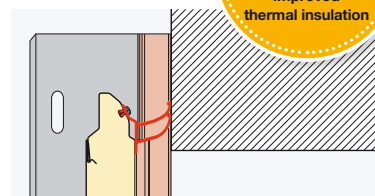
Lintel sealing
